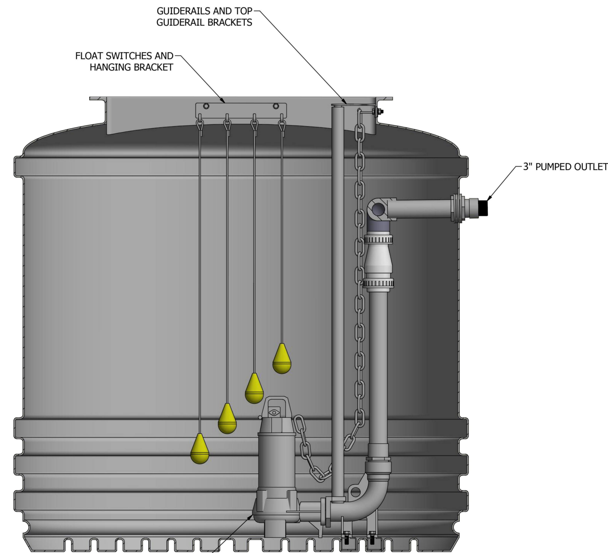
SECTION A-A SCALE 1:7.5
